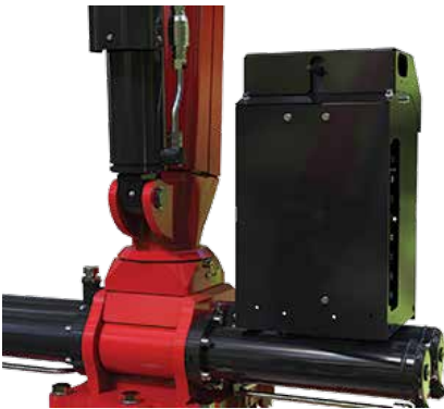
Electro-proportional control Danfos with console and 2 joysticks
